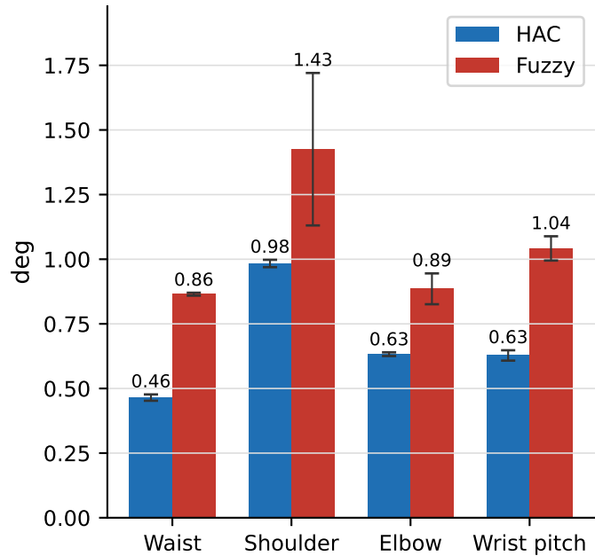
Tracking RMSE per joint
