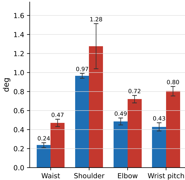
Steady-state error per joint (|e| averaged over last 1.5 s of each hold)
