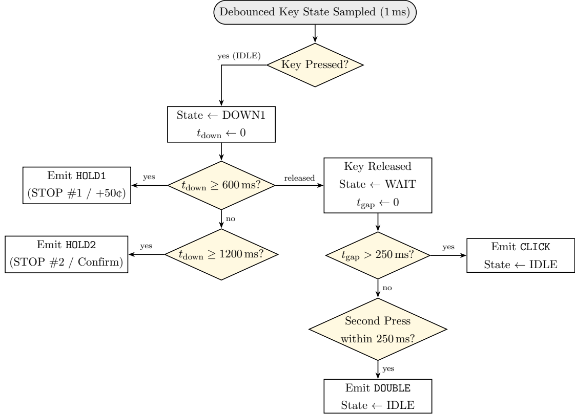
Figure 9.5: Multi-gesture button decoder sub-machine flowchart
