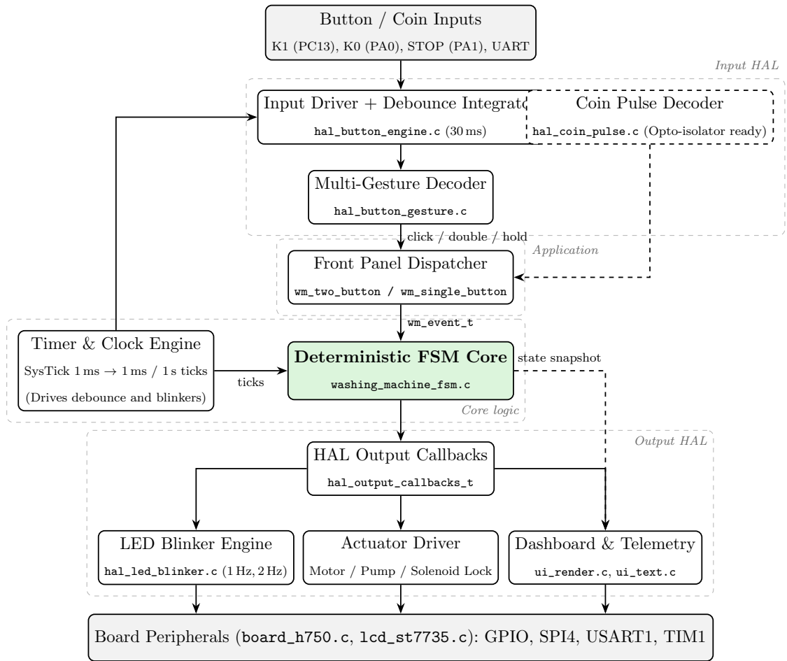
Figure 6.1: Layered software architecture of the washing machine control system
