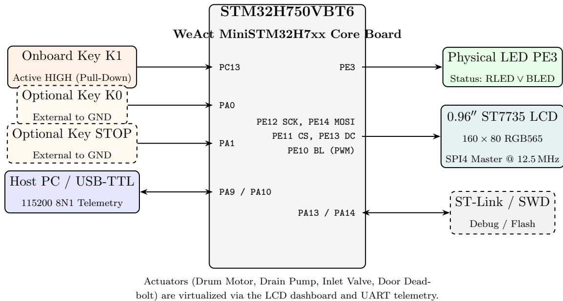
Figure 5.1: Hardware interconnect diagram of the WeAct STM32H750 implementation
