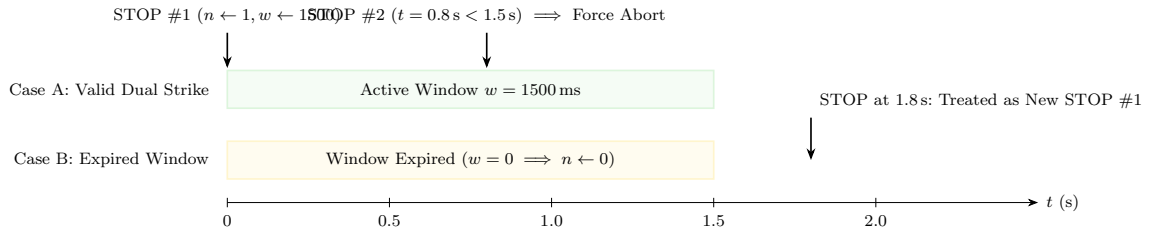
Figure 7.2: Timing geometry of the double-press STOP confirmation window
