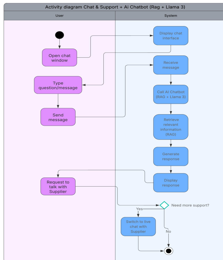
Figure 2.22. Activity diagram Chat & Support + Ai Chatbot (Rag + Llama 3)
