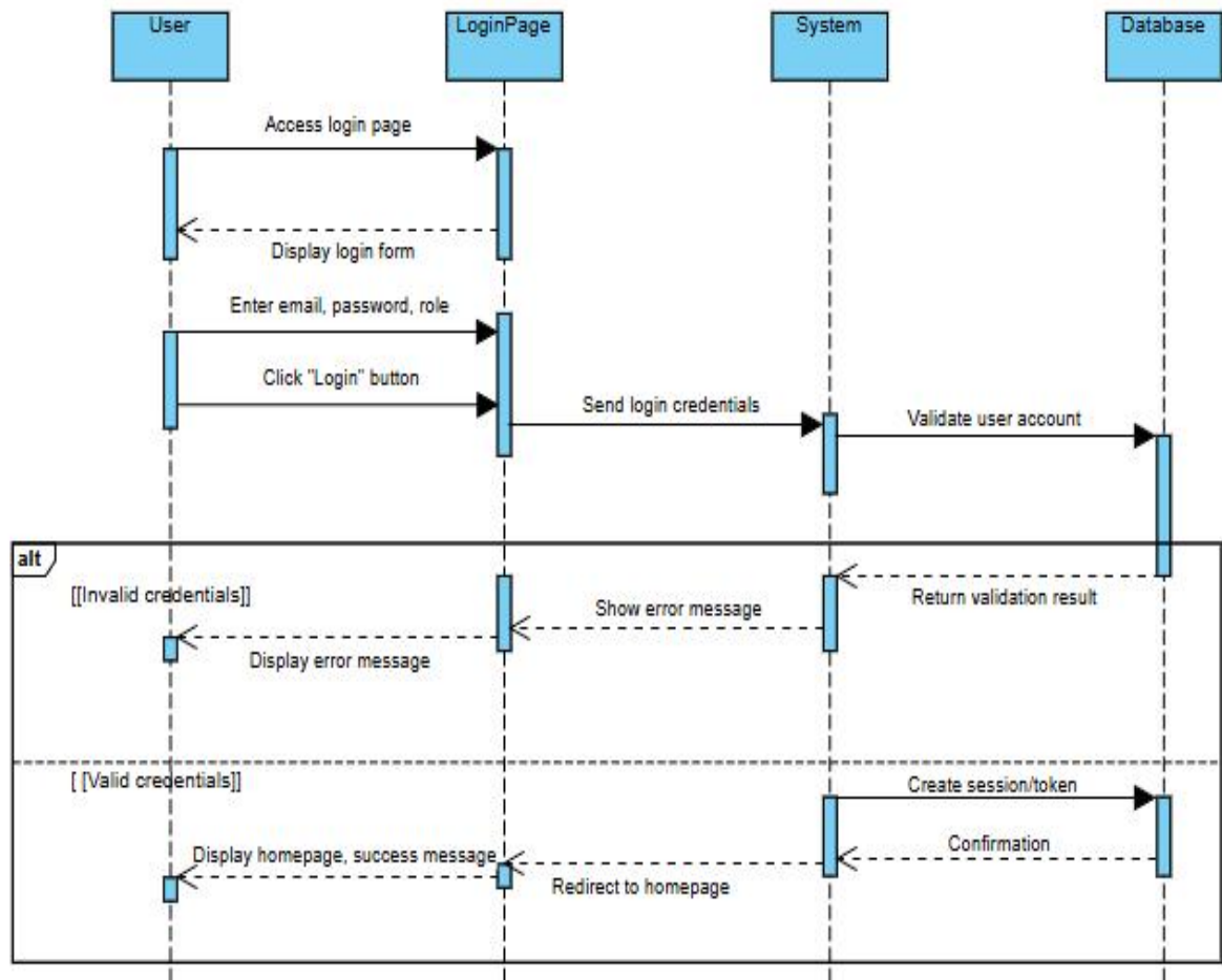
Figure 2.26. Sequence diagram Login
