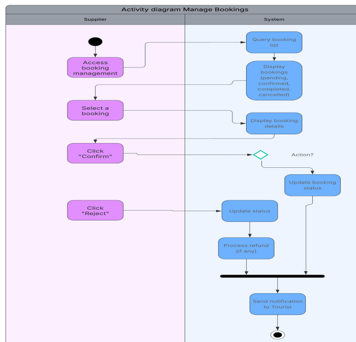
Figure 2.24. Activity diagram Manage Bookings
