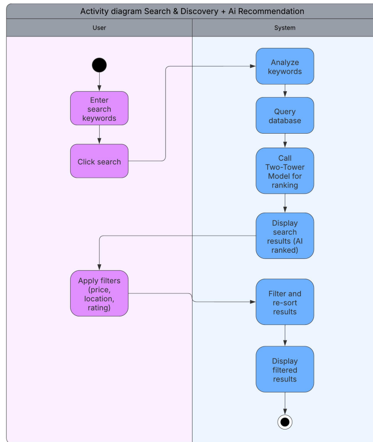
Figure 2.21. Activity diagram Search & Discovery + Ai Recommendation
