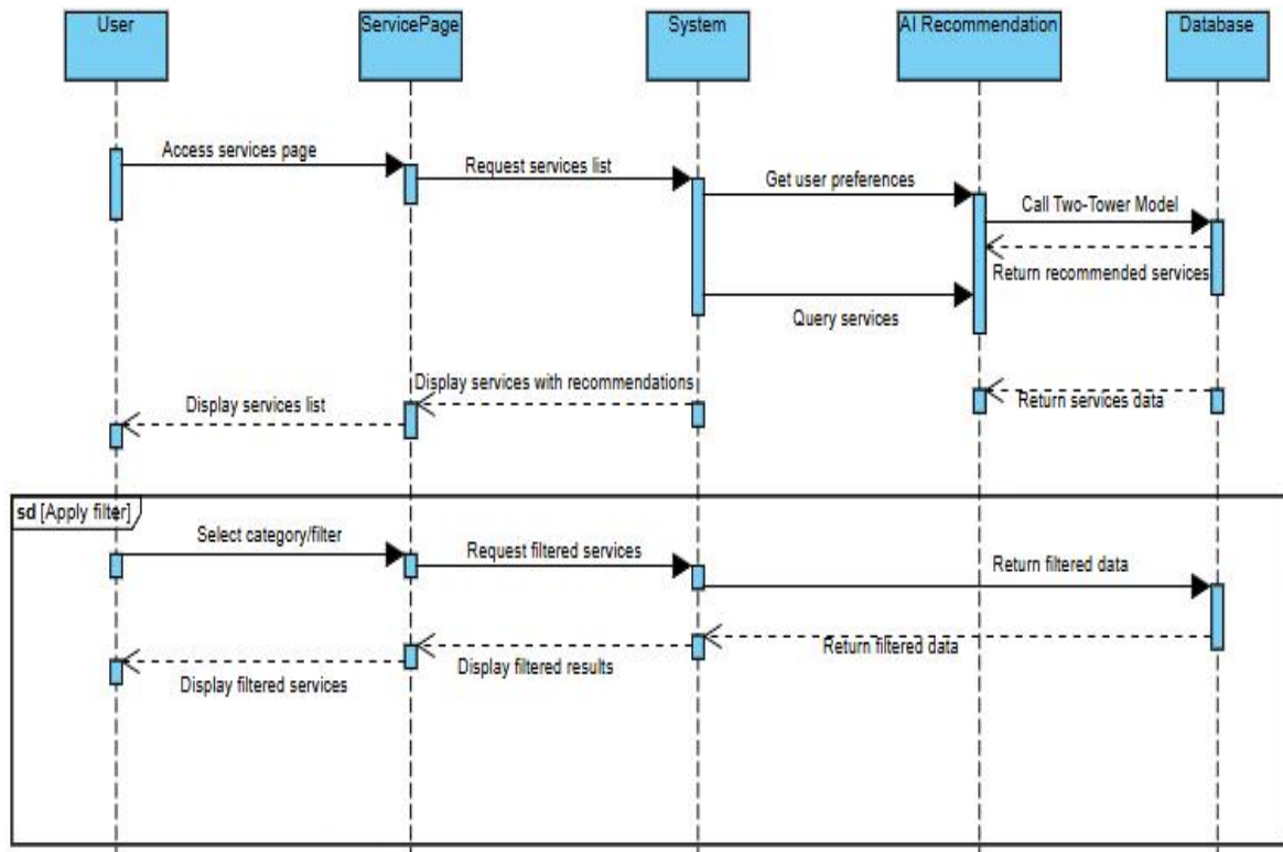
Figure 2.27. Sequence diagram Browse Services
