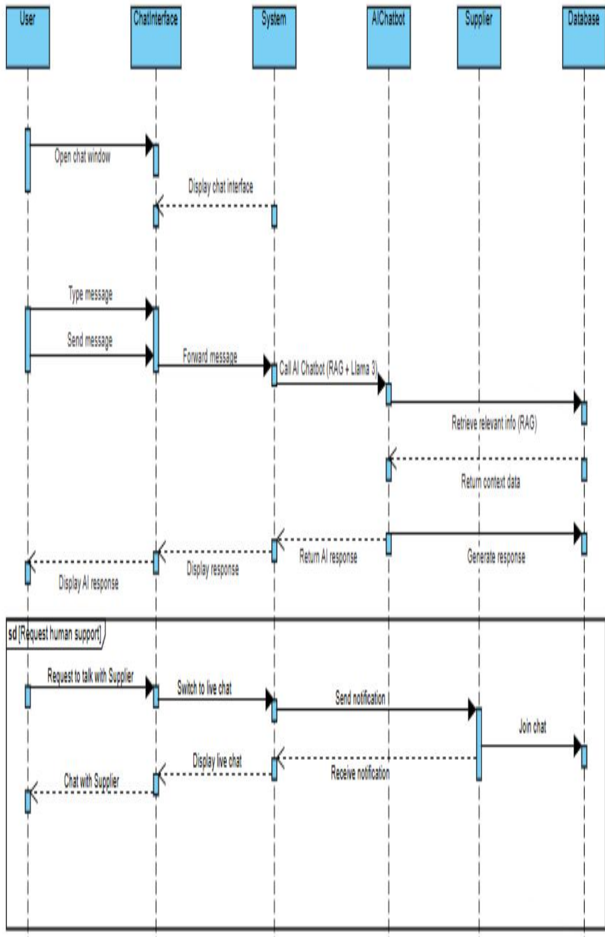
Figure 2.30. Sequence diagram Chat & Support + Ai Chatbot (Rag + Llama 3)
