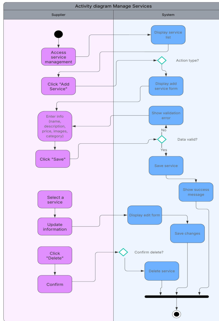
Figure 2.23. Activity diagram Manage Services
