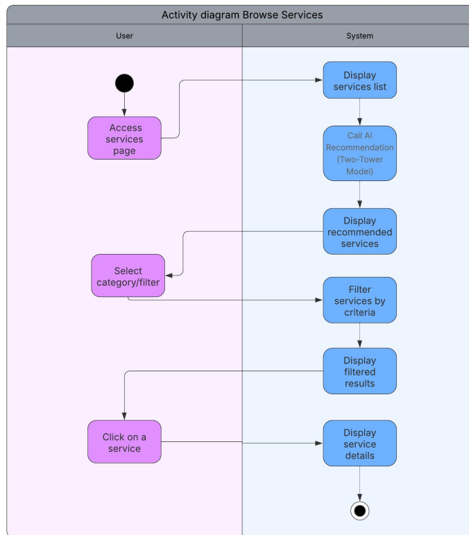
Figure 2.19. Activity diagram Browse Services
