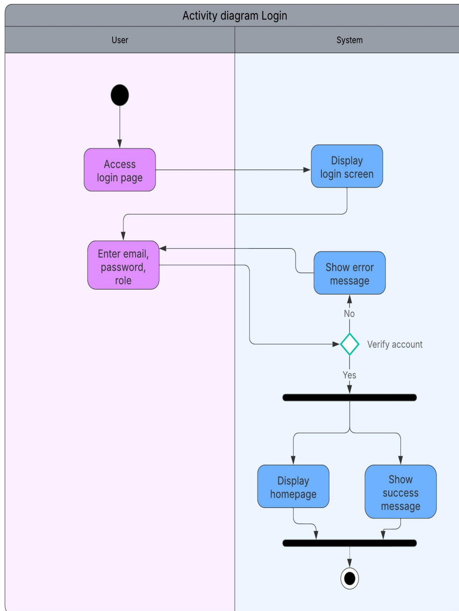
Figure 2.18. Activity diagram Login
