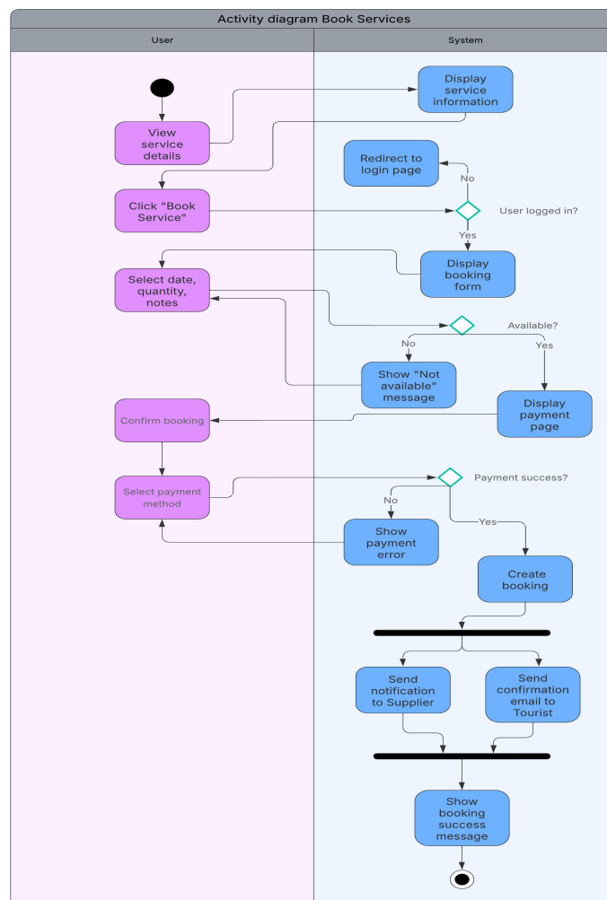
Figure 2.20. Activity diagram Book Services
