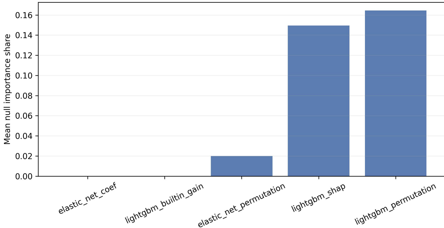
Null-feature benchmarking across importance methods
