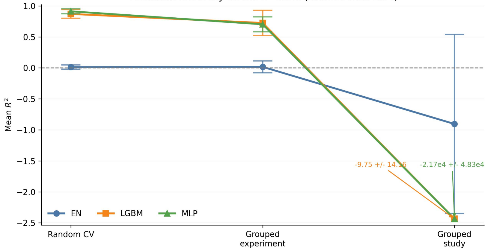
Validation hierarchy on the R^2 scale (zoomed near zero)
