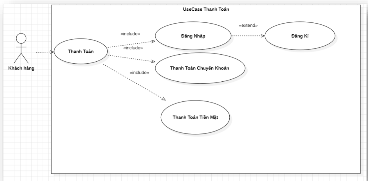
Figure 3-1: Usecase thanh toán.
