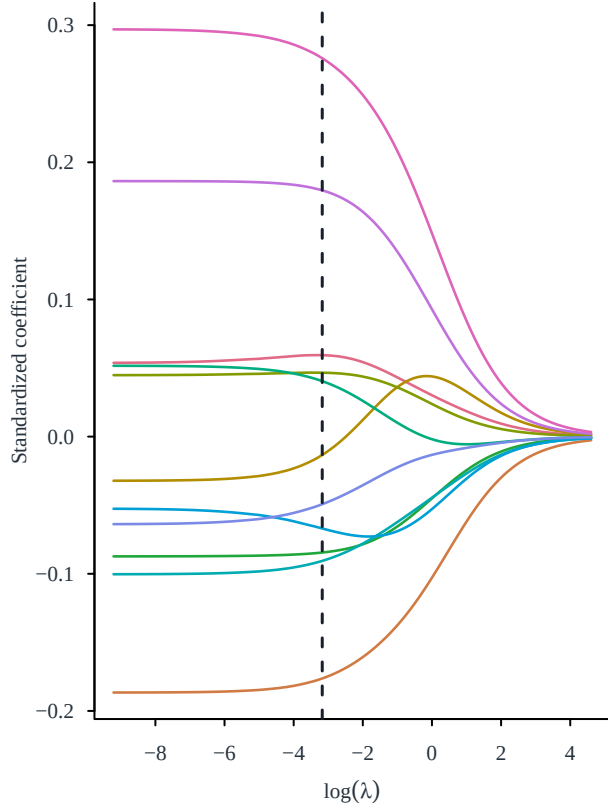
Ridge paths
