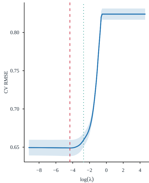
Elastic Net (alpha = 0.75)
