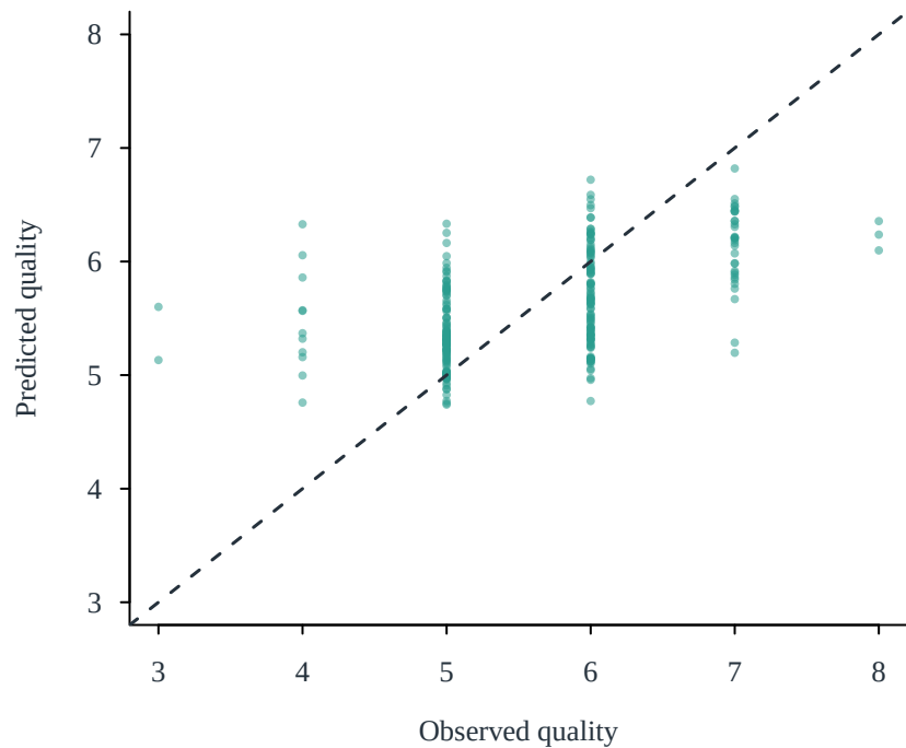
Elastic Net (RMSE 0.700)
