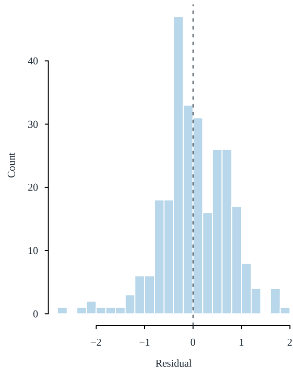
Residual distribution
