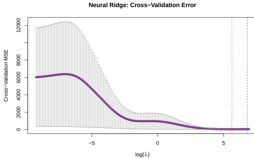
Figure 17: Shared-fold CV curve for Ridge on the fixed ReLU features.
