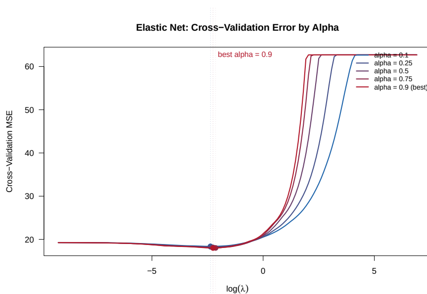
Figure 14: Elastic Net shared-fold CV performance across candidate \alpha values.
