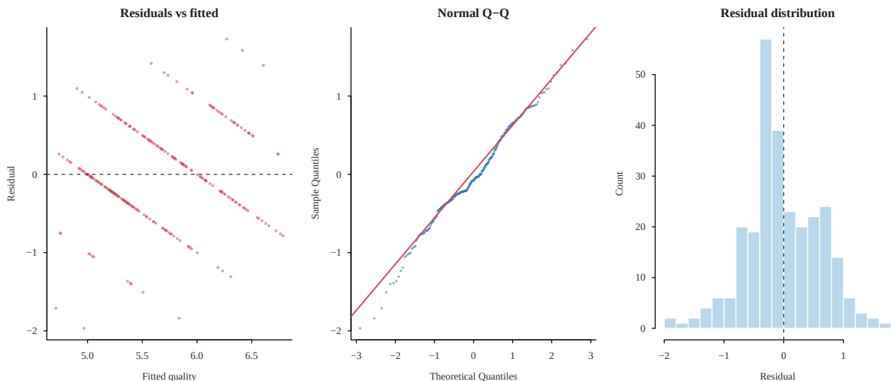
Figure 10: Residual checks for the pre-locked model on the untouched holdout set. These diagnostics describe generalization and were not used to retune the model.
