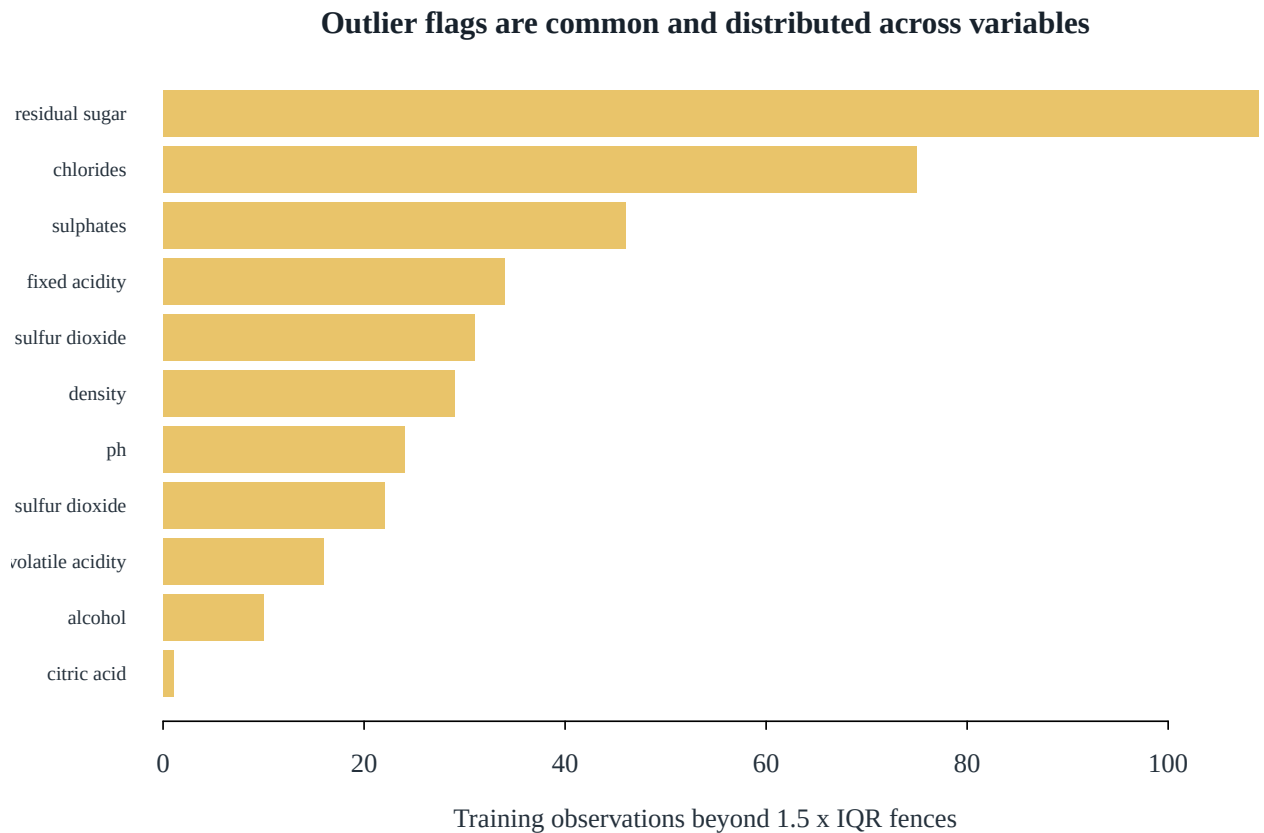
Figure 11: Training observations flagged by the univariate Tukey-IQR rule. Flags are diagnosed rather than deleted wholesale.
