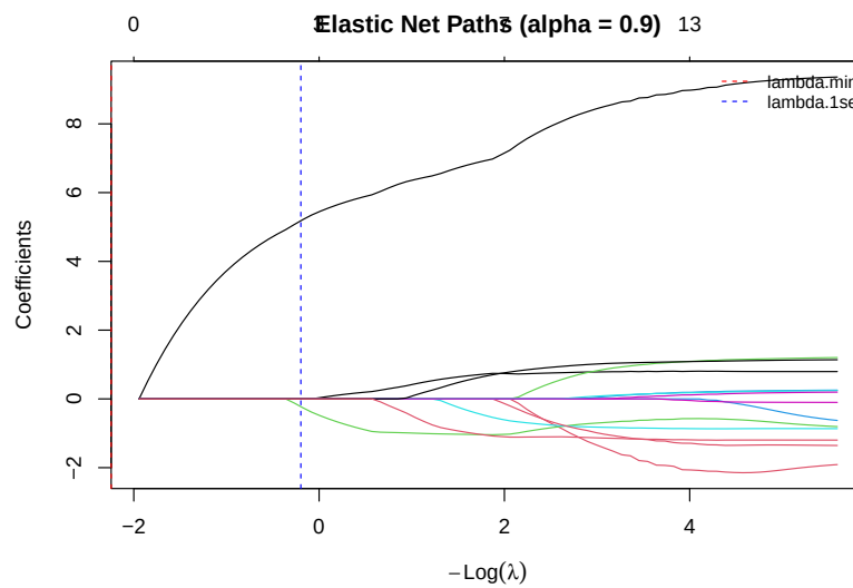
Figure 15: Elastic Net coefficient path for the selected \alpha = 0.90 .
