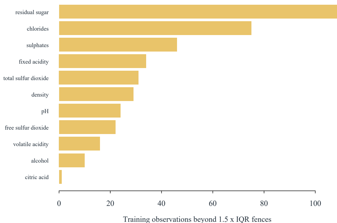
Figure 14: Training observations flagged by the univariate Tukey-IQR rule. Flags are diagnosed rather than deleted wholesale.
