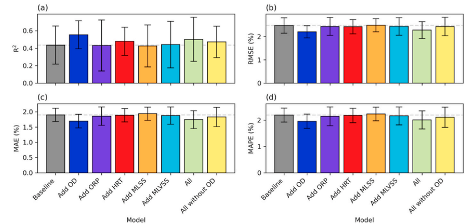
Fig. 4. Model performance with different input features. Baseline indicates using T-R, T-in, T-env, pH-in, COD-in, and flux as features. Error bar is the 95% confidence intervals of the error metrics from 10-fold cross validation.
