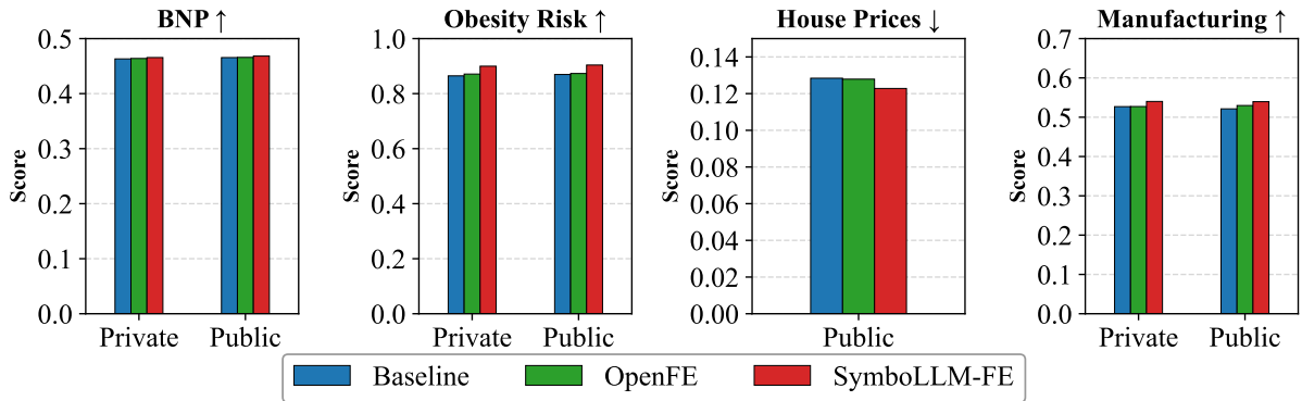
Figure 3: Score comparison on Kaggle competitions. ' \uparrow ' means classification and ' \downarrow ' means regression.
