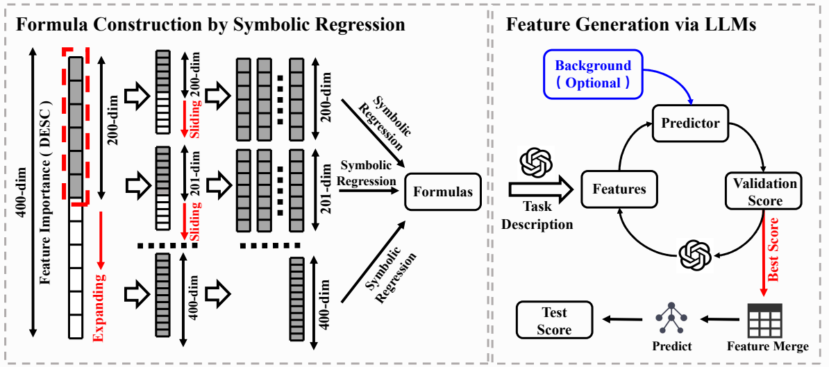
Figure 2: Overview of SymbolLLM-FE, including Formula Construction by Symbolic Regression and Feature Generation via LLMs and downstream predictors.
