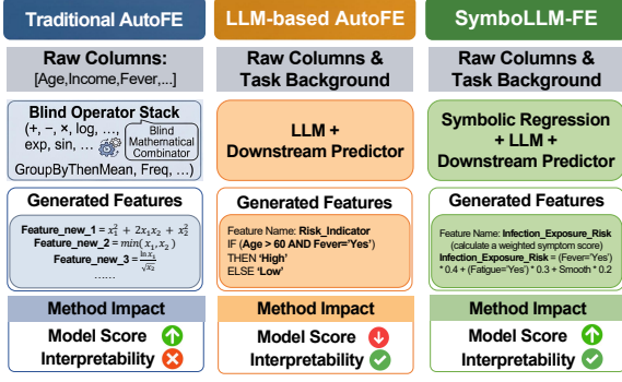
Figure 1: Comparative analysis of feature generation mechanisms and interpretability paradigms across AutoFE. Traditional AutoFE rely on blind operator stacks, yielding high performance but poor interpretability. LLM-based AutoFE offer semantic clarity but may suffer from performance instability. Our proposed SymboLLM-FE synergizes symbolic regression with LLMs to achieve both high predictive accuracy and human-interpretable transparency.
