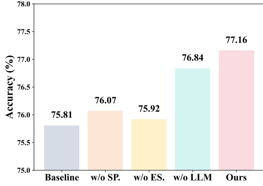
Figure 4: Ablation study. SP. means Spearman-value-based feature pre-sorting. ES. means the expanding-sliding window approach. LLM means LLM-based feature generation.
