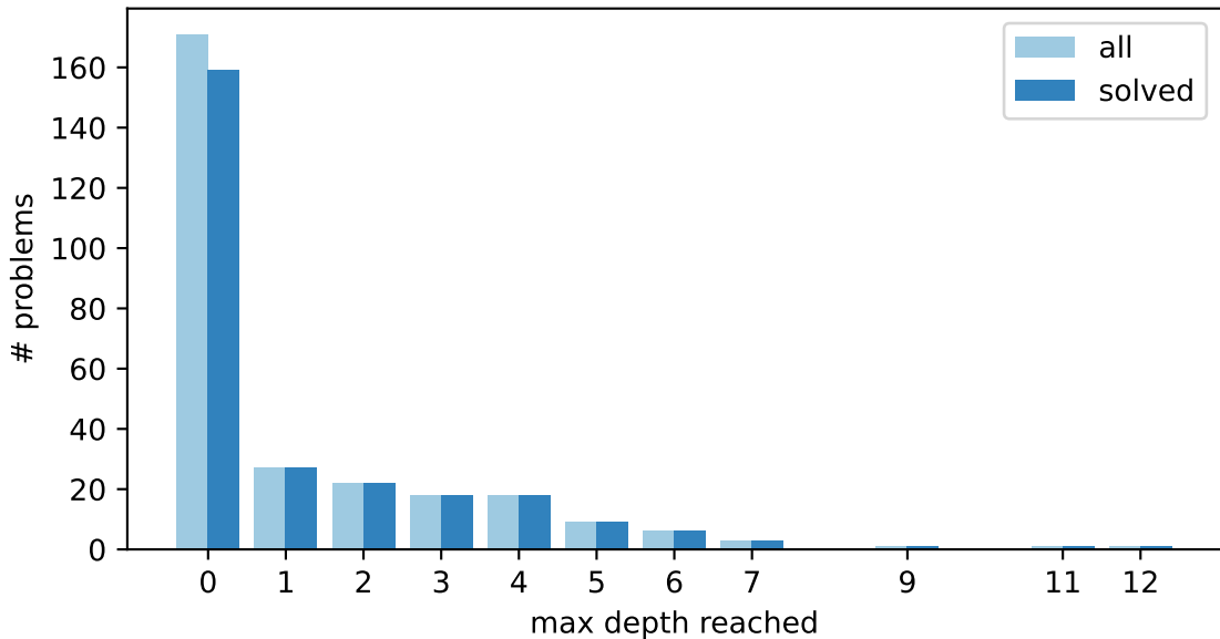
Search depth distribution (GammaZero)
