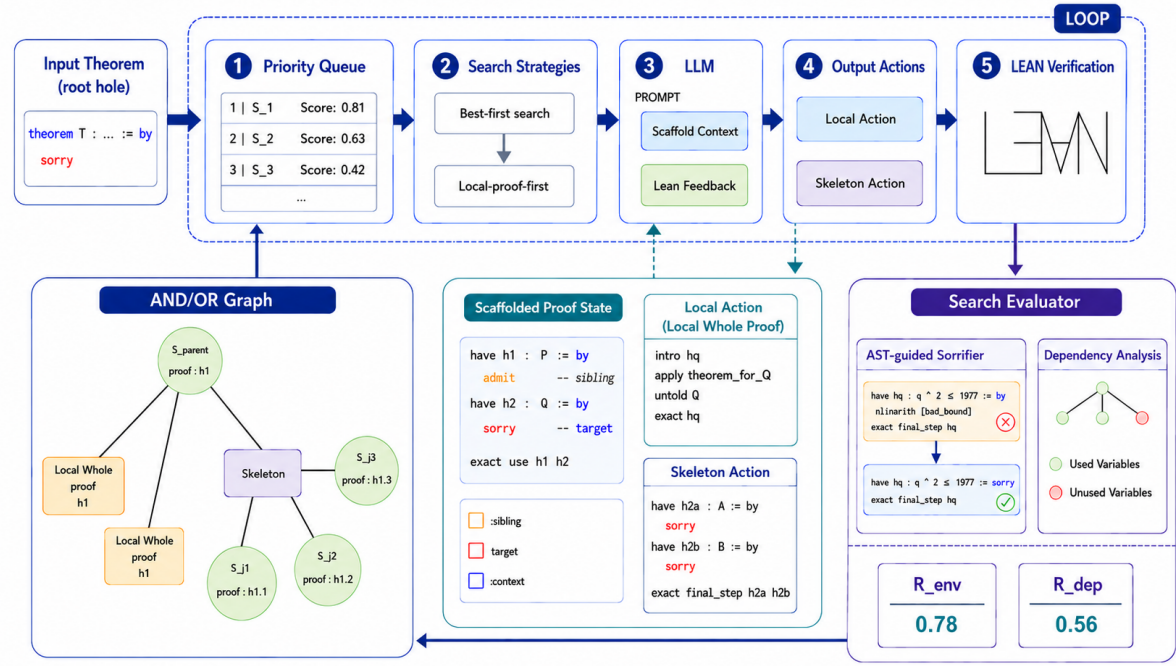
Figure 7.1.1: Overview of the GammaZero framework. The system maintains a priority queue over scaffolded proof states, asks the LLM for local proof or skeleton actions, checks candidates with Lean, applies AST-guided patching when useful, computes syntactic and dependency-based scores, and updates the AND/OR proof-search graph.
