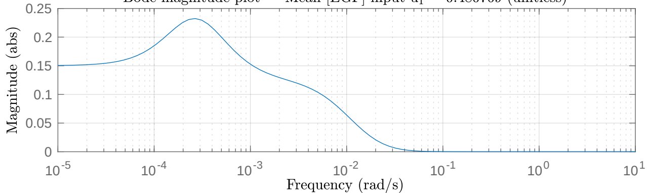
Bode magnitude plot — Mean [EGF] input u_1 = 0.480769 (unitless)
