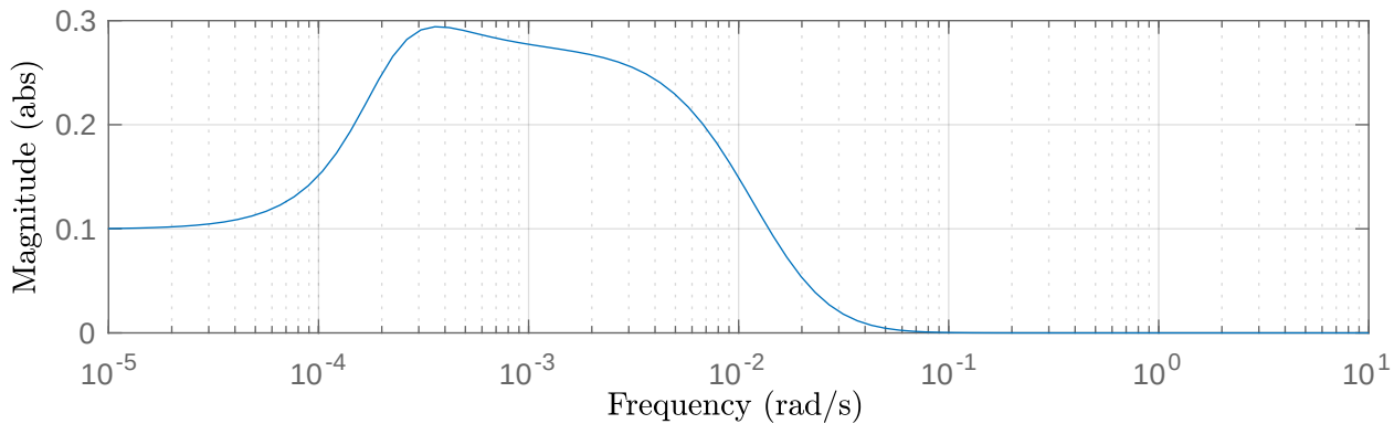
Bode magnitude plot — Mean [EGF] input u_1 = 0.271739 (unitless)
