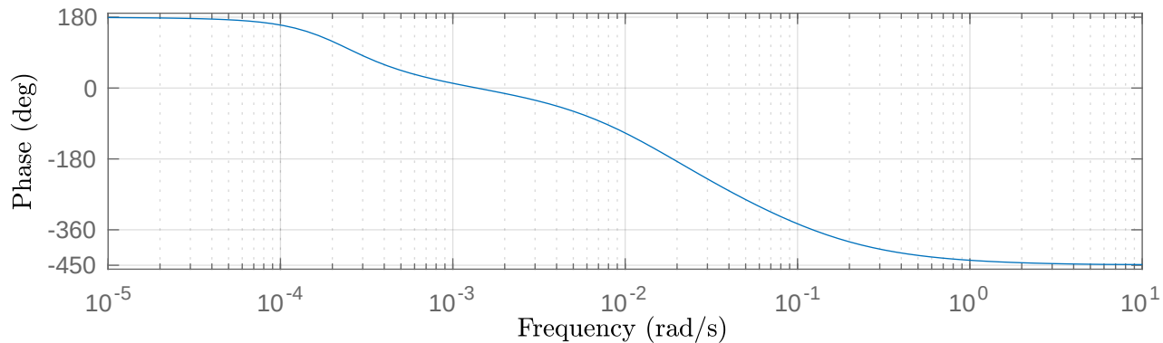
Bode phase plot — Mean [EGF] input u_1 = 0.271739 (unitless)
