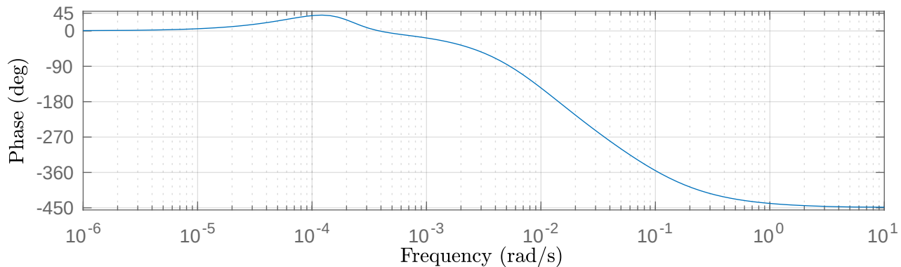
Bode phase plot — Mean [EGF] input u_1 = 0.0416667 (unitless)
