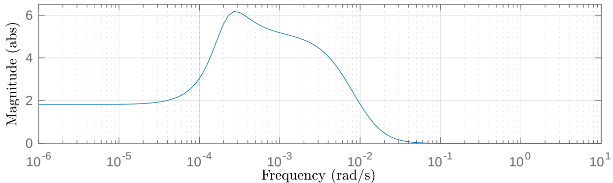
Bode magnitude plot — Mean [EGF] input u_1 = 0.0416667 (unitless)
