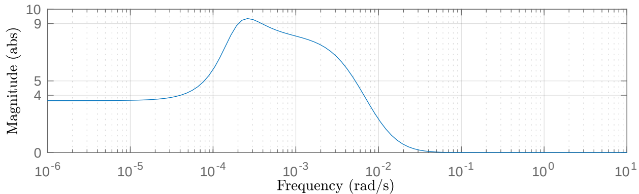
Bode magnitude plot — Mean [EGF] input u_1 = 0.0192308 (unitless)
