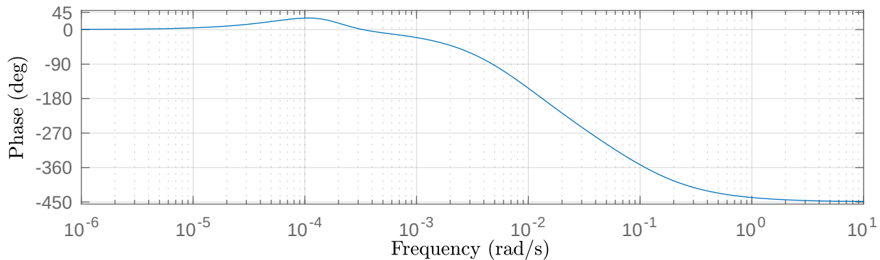
Bode phase plot — Mean [EGF] input u_1 = 0.0192308 (unitless)
