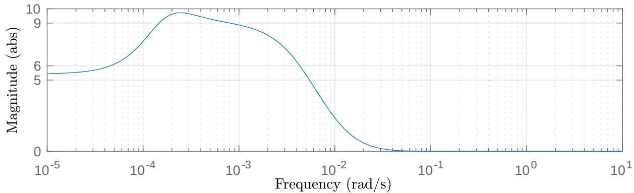
Bode magnitude plot — Mean [EGF] input u_1 = 0.0108696 (unitless)
