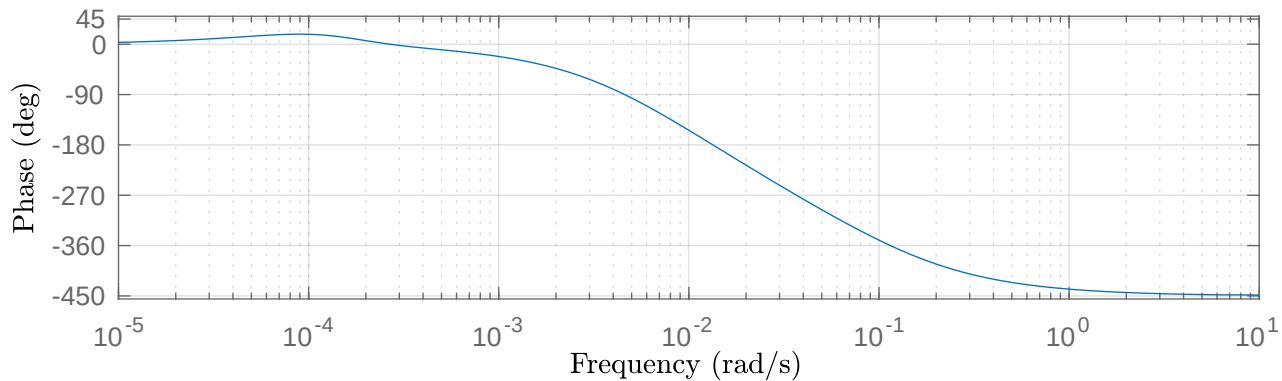
Bode phase plot — Mean [EGF] input u_1 = 0.0108696 (unitless)
