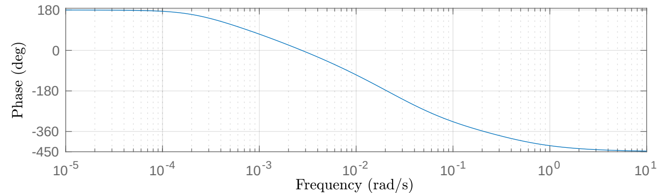
Bode phase plot — Mean [EGF] input u_1 = 2.08333 (unitless)
