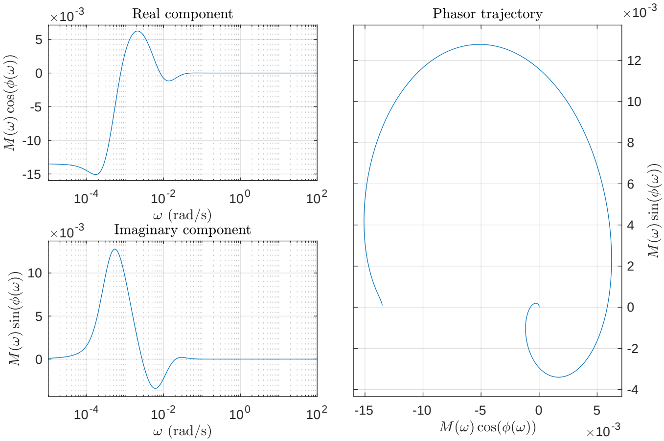
Phasor Trajectory — Mean [EGF] input u_1 = 2.08 Kd
