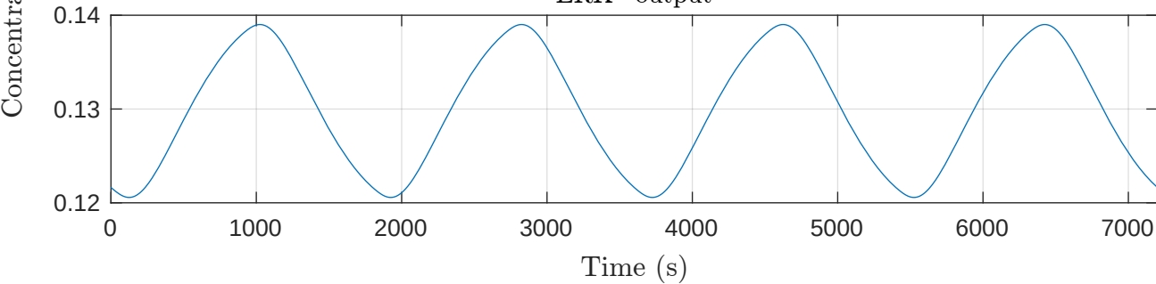
ERK* output
