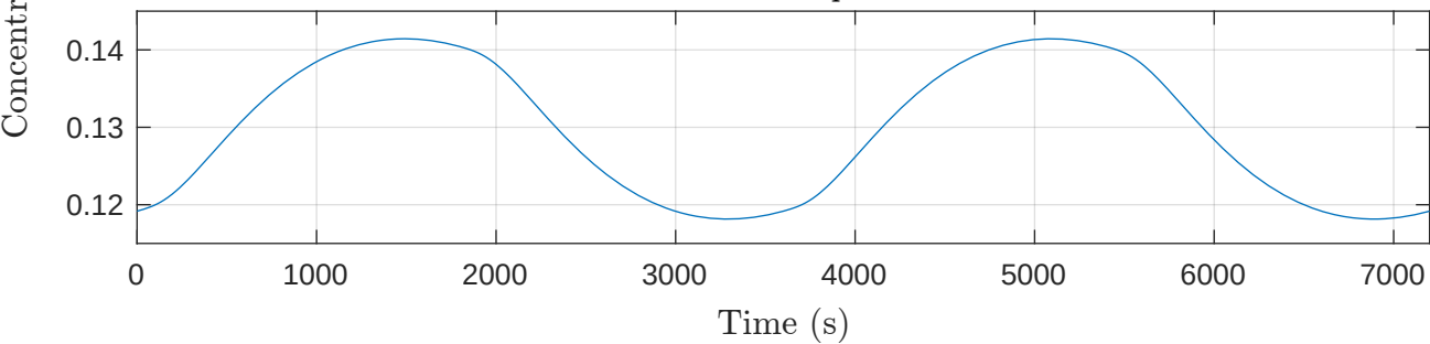
ERK* output
