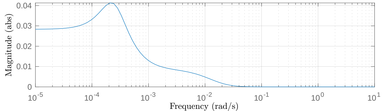
Bode magnitude plot — Mean [NGF] input u_1 = 0.961538 (unitless)
