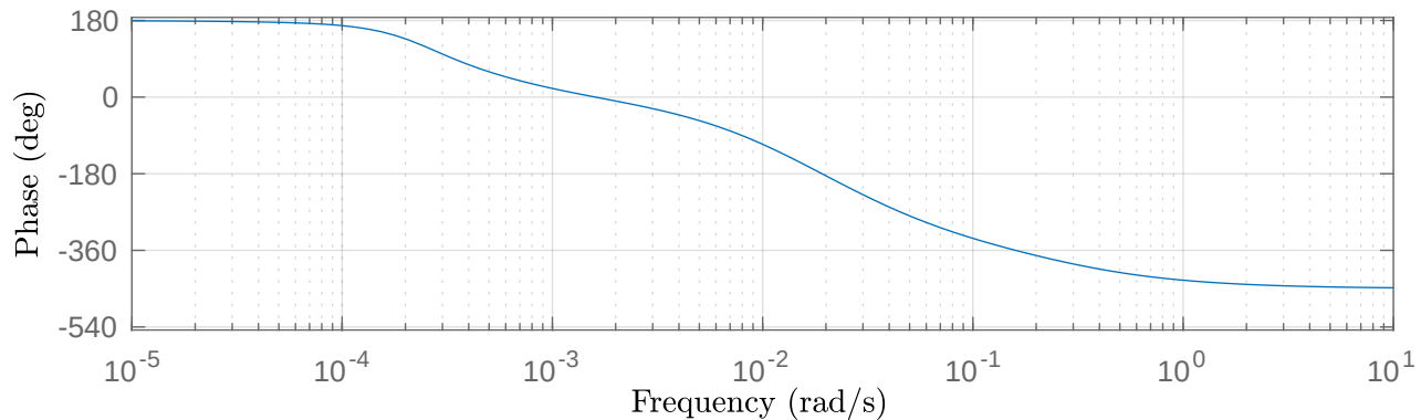
Bode phase plot — Mean NGF input u_1 = 0.961538 (unitless)
