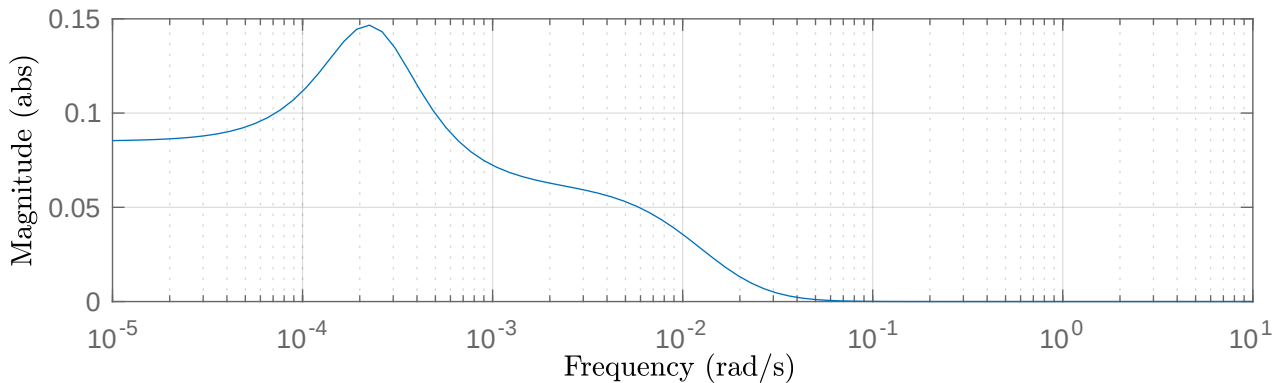
Bode magnitude plot — Mean [NGF] input u_1 = 0.443787 (unitless)
