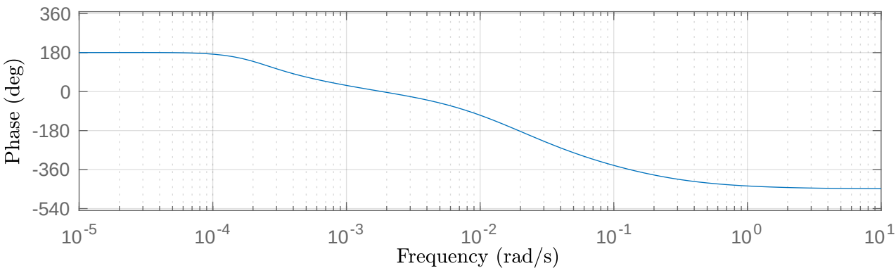
Bode phase plot — Mean NGF input u_1 = 0.443787 (unitless)
