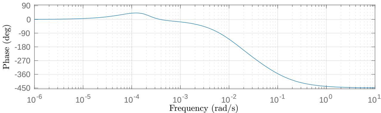
Bode phase plot — Mean NGF input u_1 = 0.0915751 (unitless)
