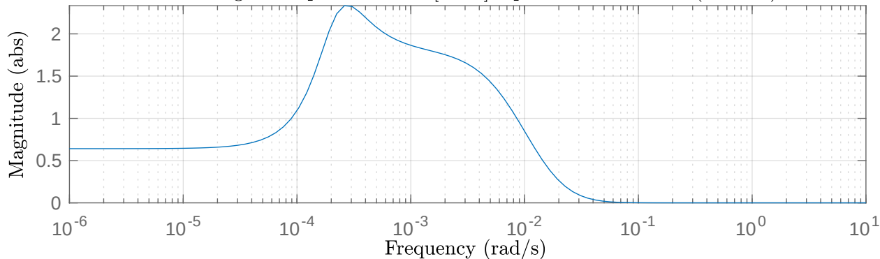
Bode magnitude plot — Mean [NGF] input u_1 = 0.0915751 (unitless)
