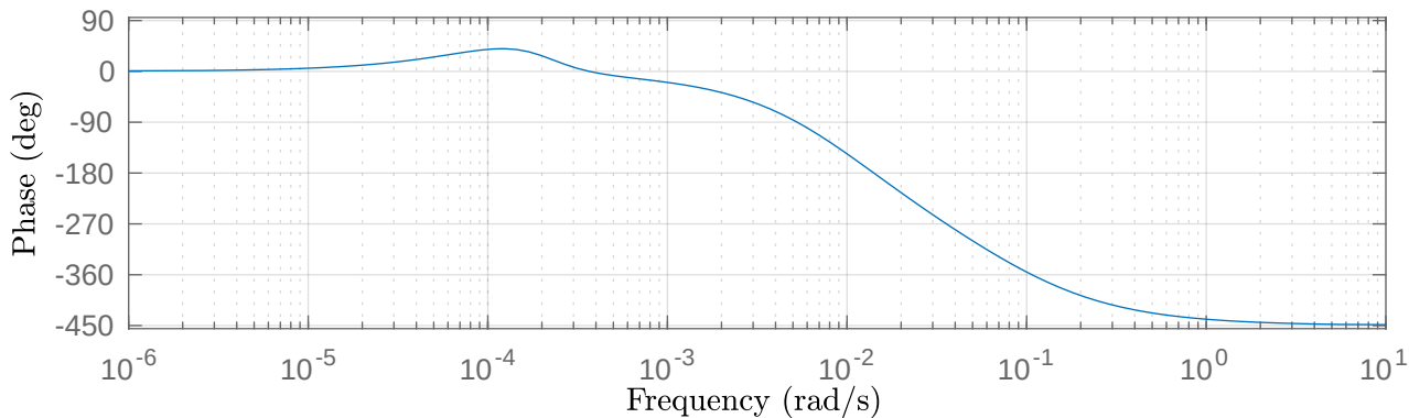
Bode phase plot — Mean NGF input u_1 = 0.0384615 (unitless)
