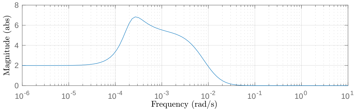
Bode magnitude plot — Mean [NGF] input u_1 = 0.0384615 (unitless)
