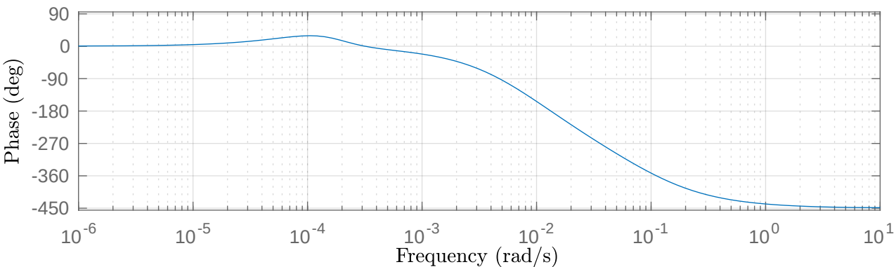
Bode phase plot — Mean NGF input u_1 = 0.0177515 (unitless)
