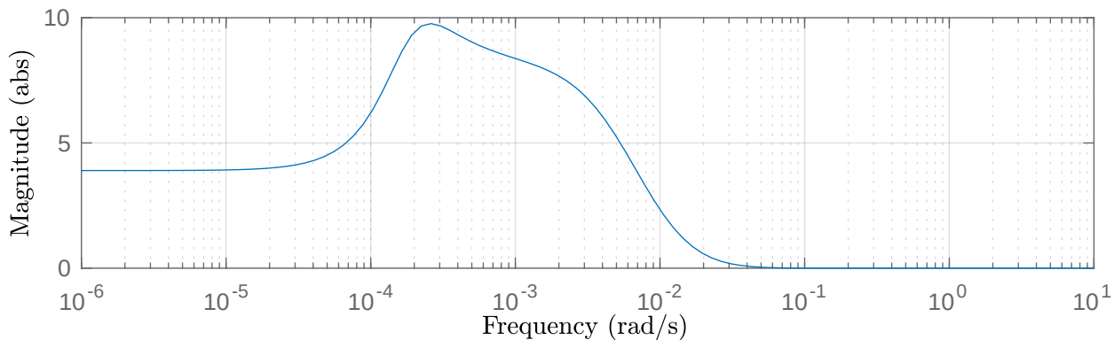
Bode magnitude plot — Mean [NGF] input u_1 = 0.0177515 (unitless)
