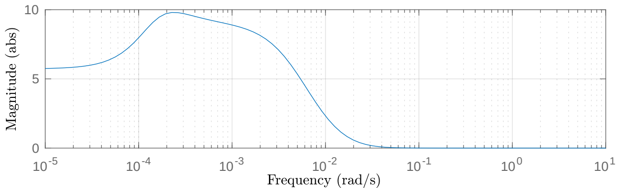
Bode magnitude plot — Mean [NGF] input u_1 = 0.0100334 (unitless)
