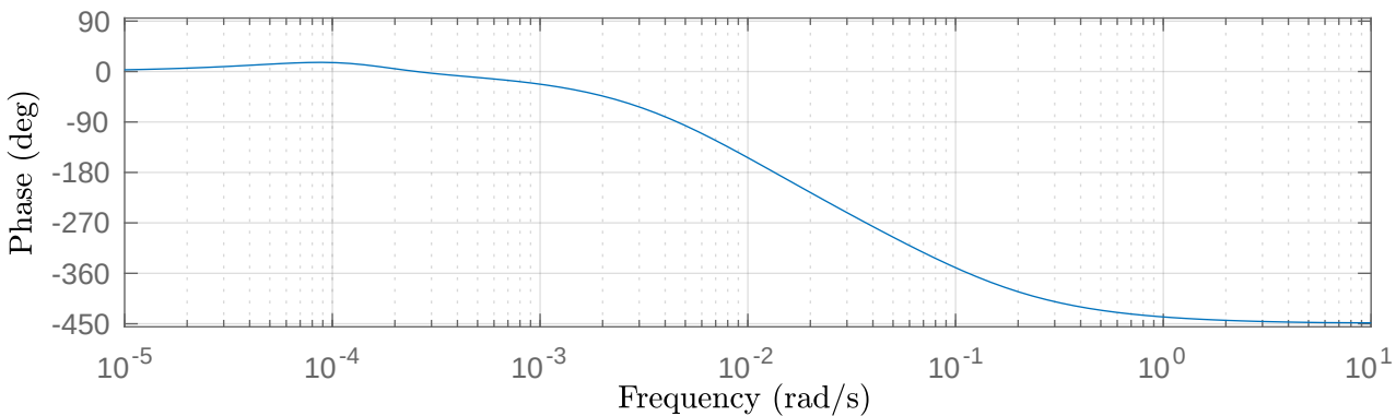
Bode phase plot — Mean NGF input u_1 = 0.0100334 (unitless)
