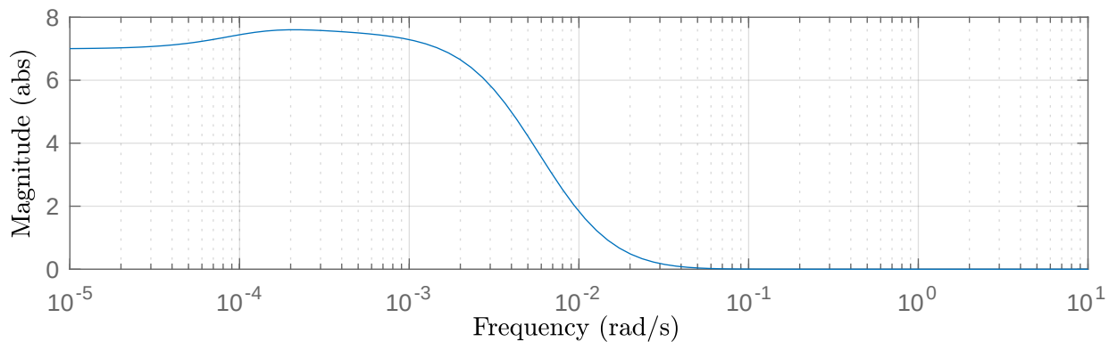
Bode magnitude plot — Mean [NGF] input u_1 = 0.003663 (unitless)
