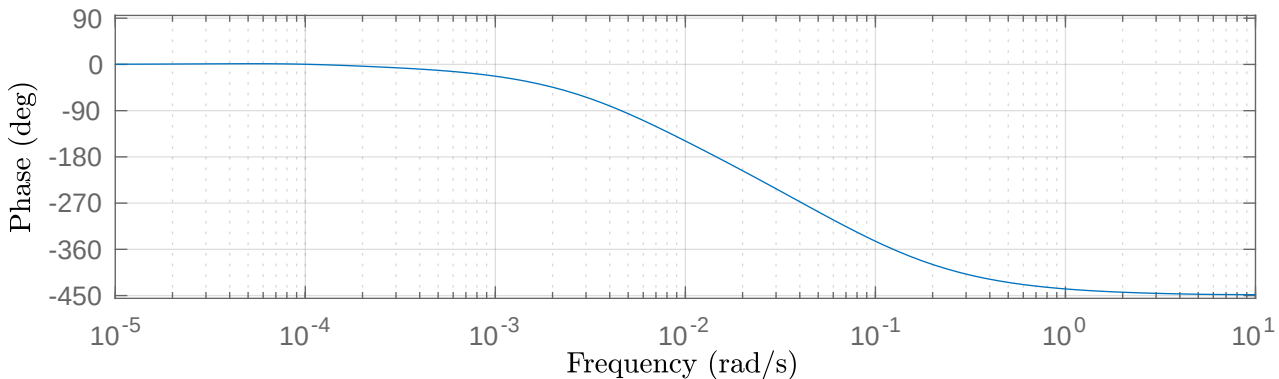
Bode phase plot — Mean NGF input u_1 = 0.003663 (unitless)
