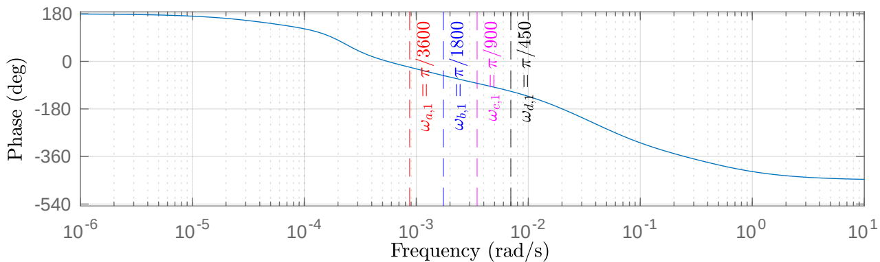
Bode phase plot — Constant [NGF] input u_1 = 5.76923 Kd
