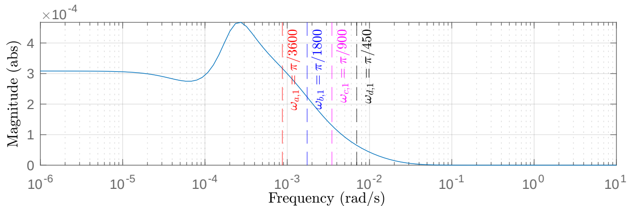
Bode magnitude plot — Constant [NGF] input u_1 = 5.76923 Kd
