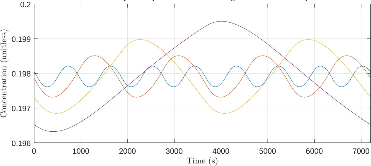
ERK* Output Responses to NGF Triangular Pulse Train Inputs
