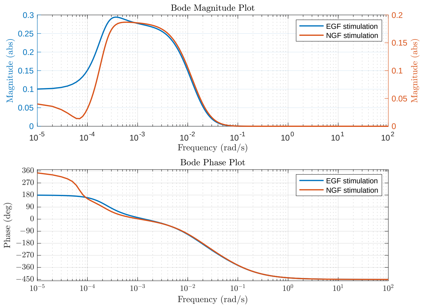
Bode Plots Corresponding to Moderate EGF and NGF Stimulation (0.25 Kd)
