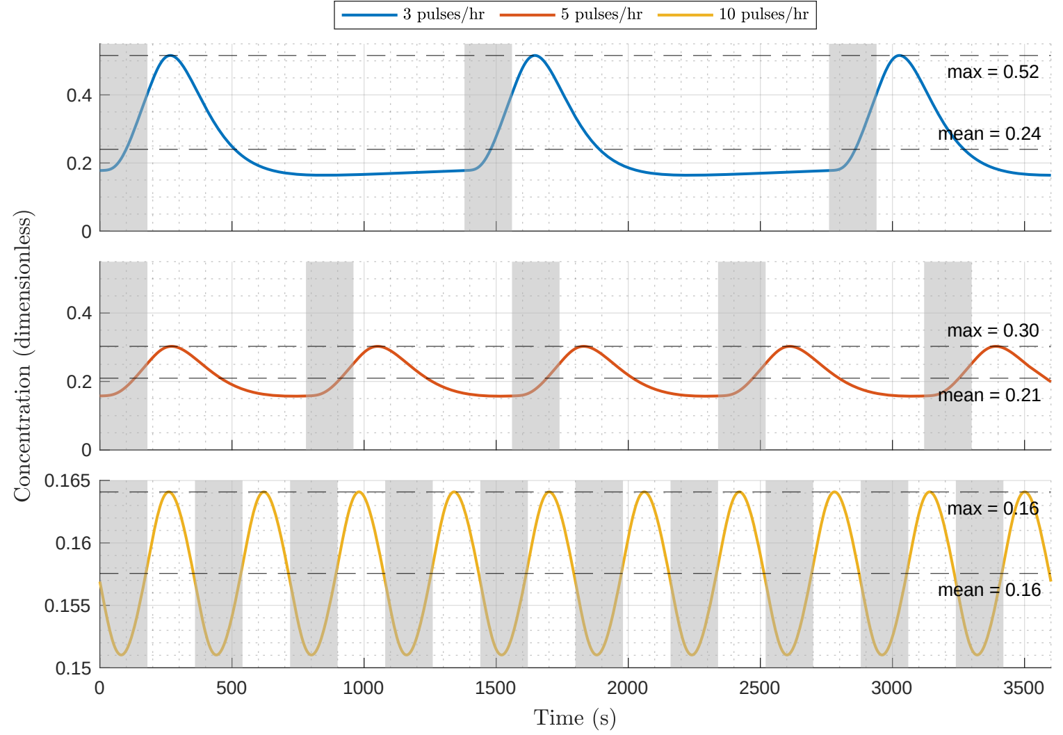
Simulated ERK* Output Kinetics for Periodic Rectangular EGF Input Pulses of 2.1 Kd
