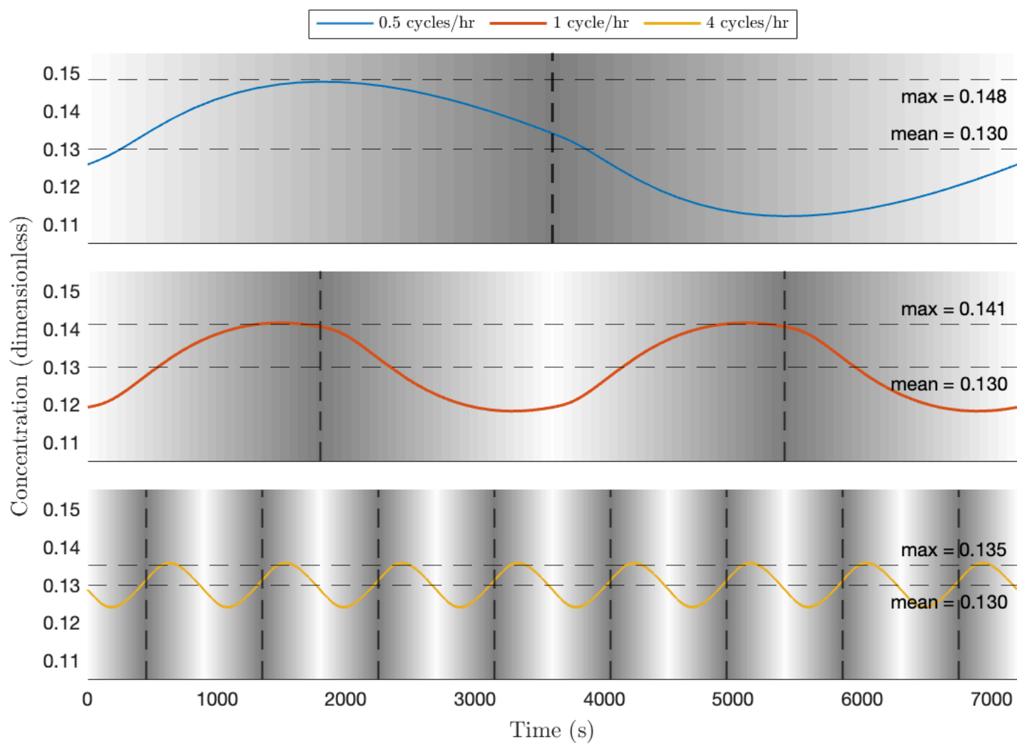
Simulated ERK* Output Kinetics for Periodic Triangular EGF Input Pulses of 4.2 Kd
