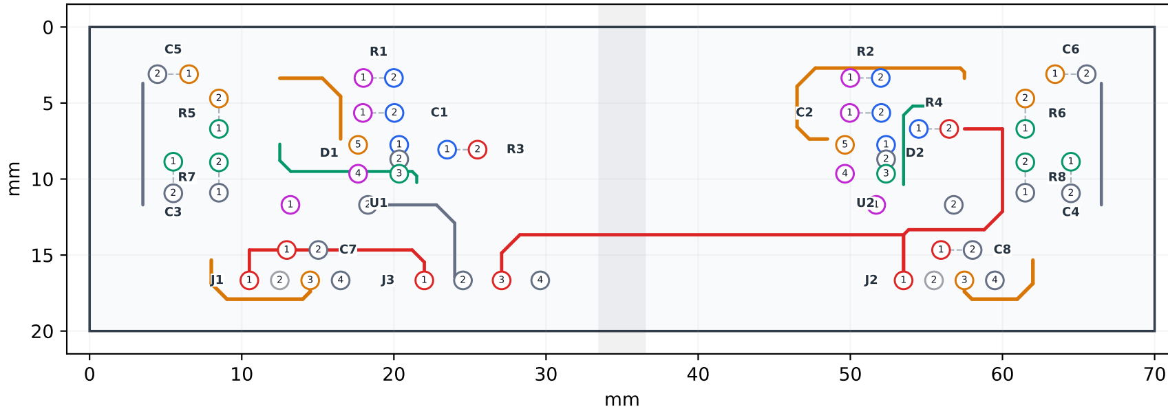
Top copper / through-hole wiring
