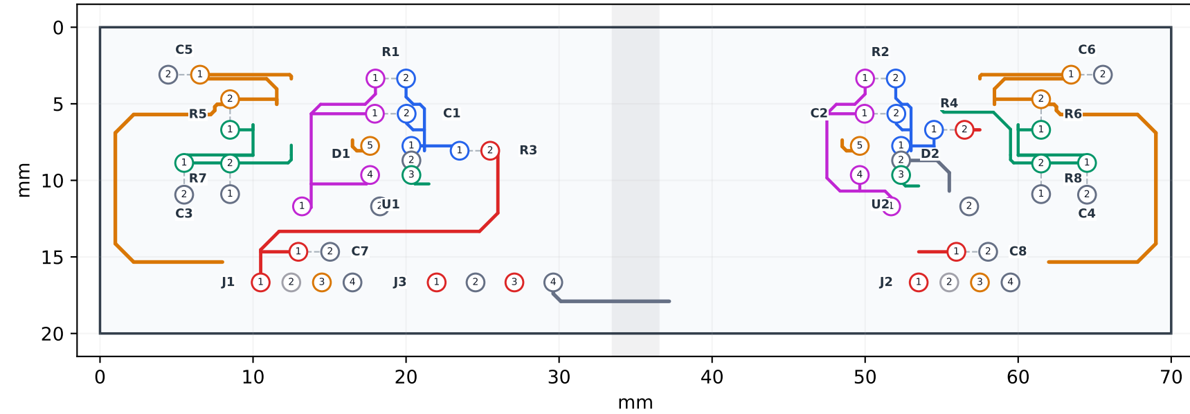
Rear analog layout / B.Cu viewed from top
