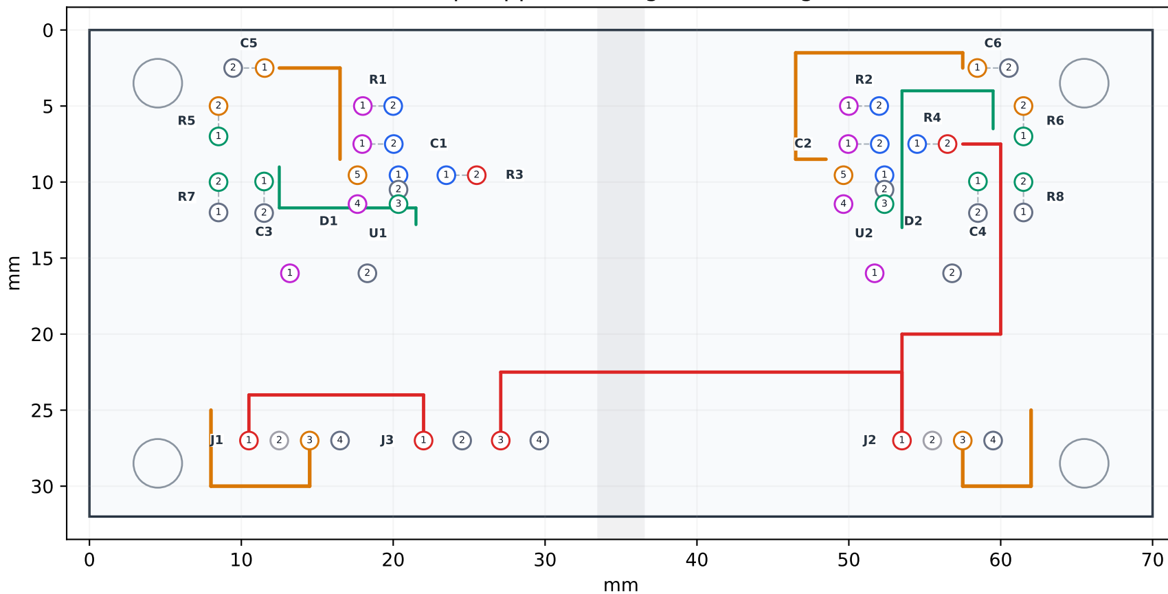
Top copper / through-hole wiring
