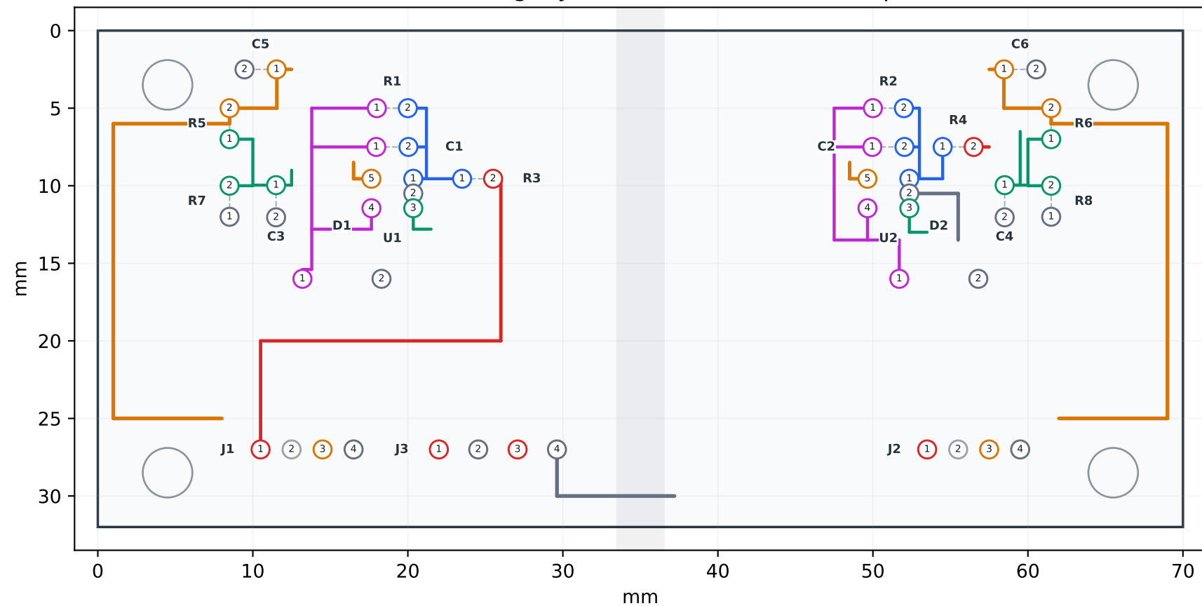
Rear analog layout / B.Cu viewed from top
