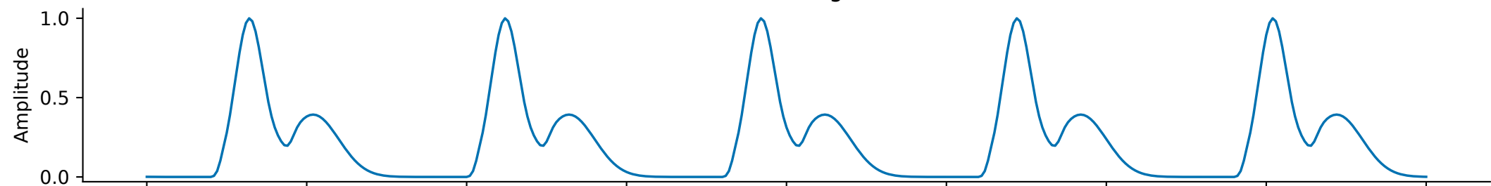
Gaussian (fitted)
