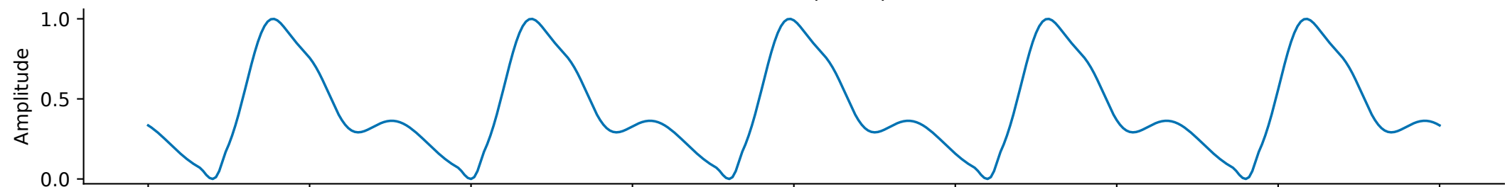
cWGAN-GP
