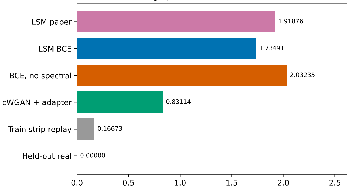
Mean log-spectrum RMSE (lower is better)
