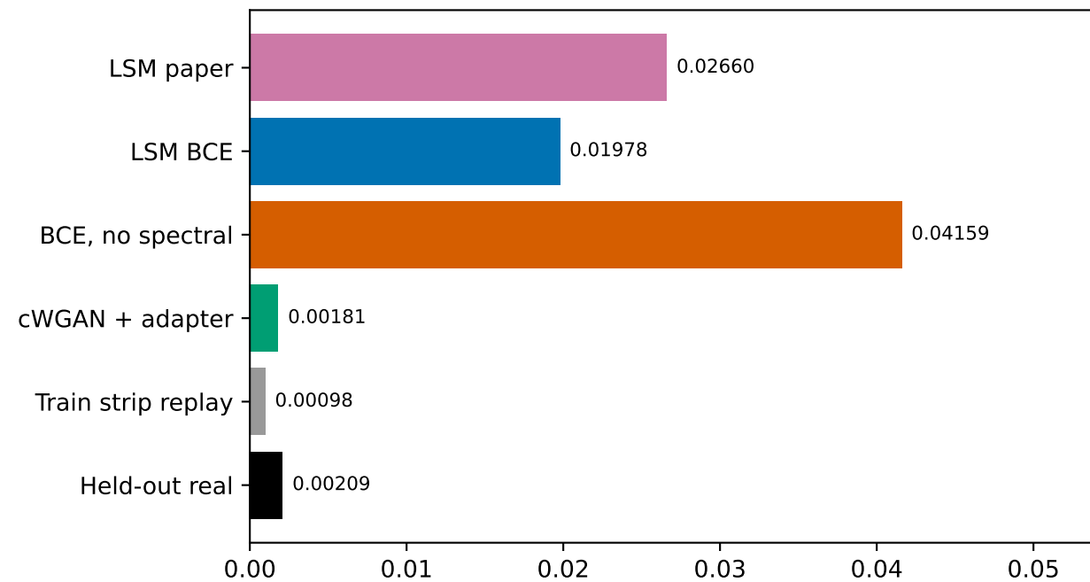
Power above 5 Hz (%)
