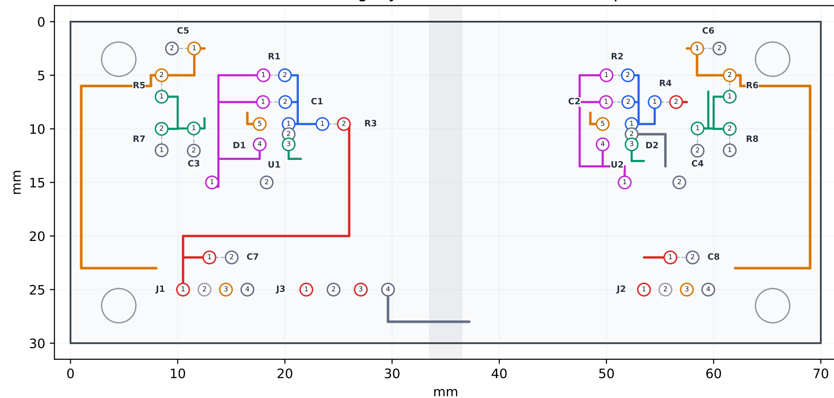
Rear analog layout / B.Cu viewed from top
