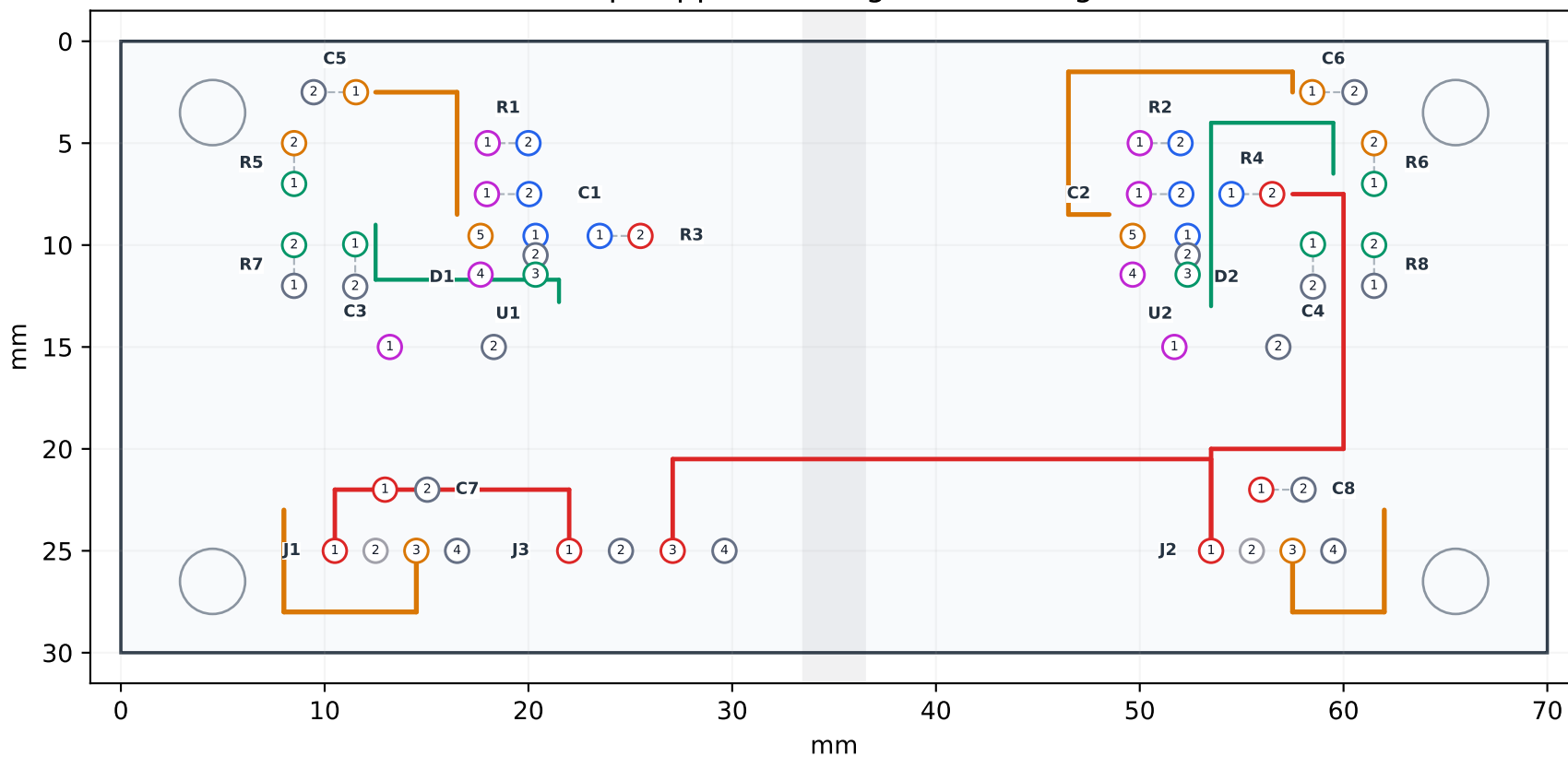
Top copper / through-hole wiring
