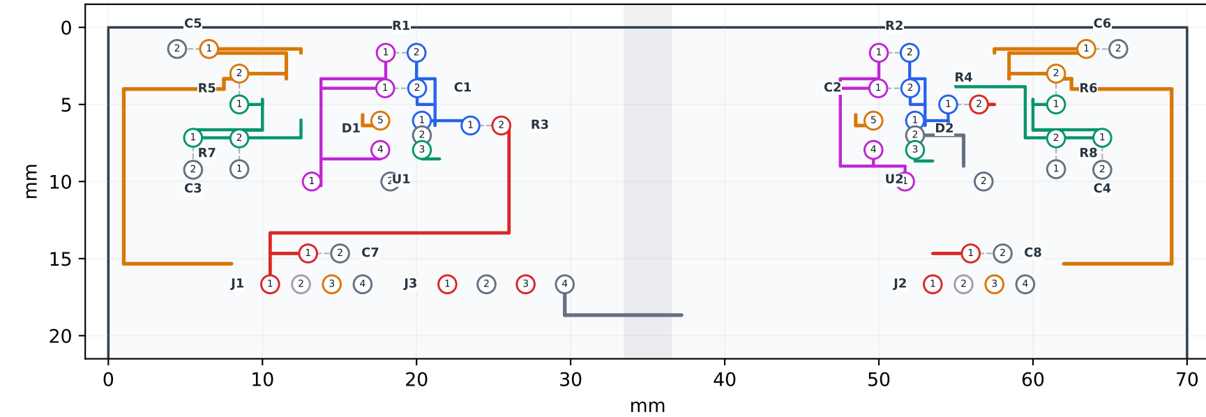
Rear analog layout / B.Cu viewed from top
