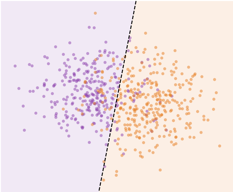
Seasonality CSS = 78.6% ✓
