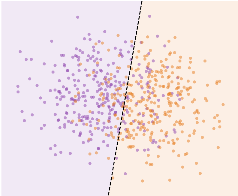
Volatility CSS = 70.9% ✓
