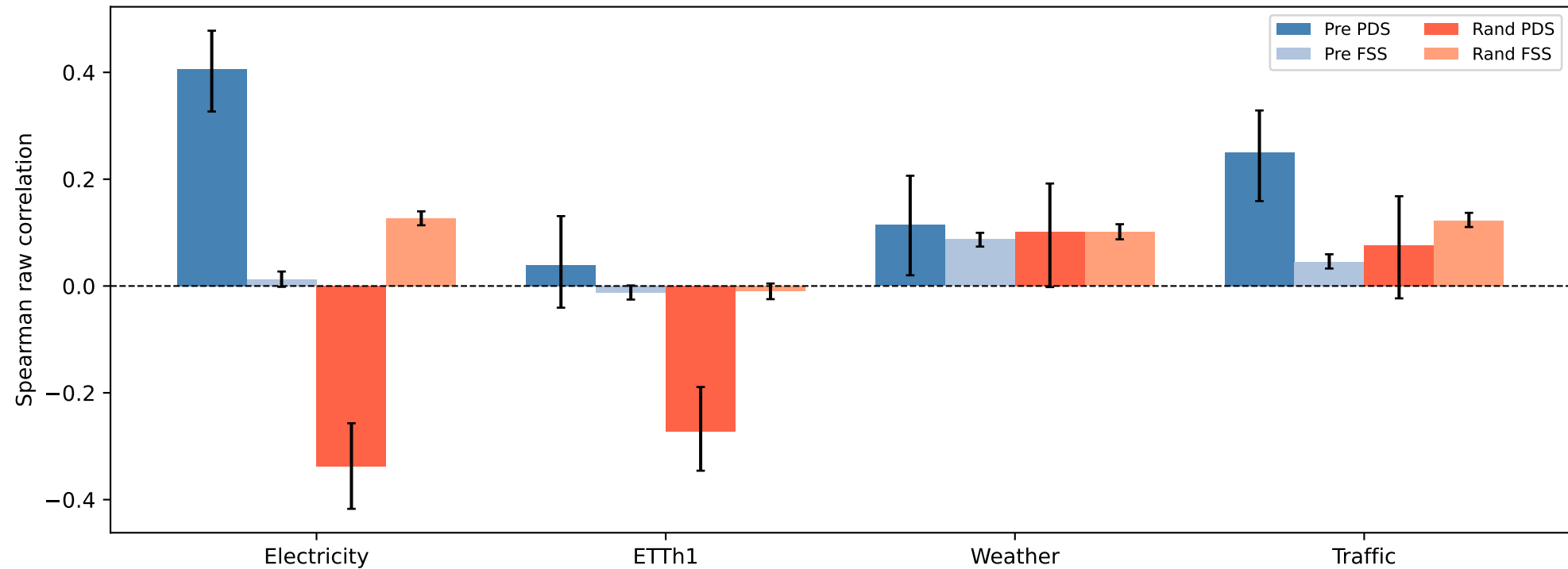
Geodesic reliability: PDS vs FSS
