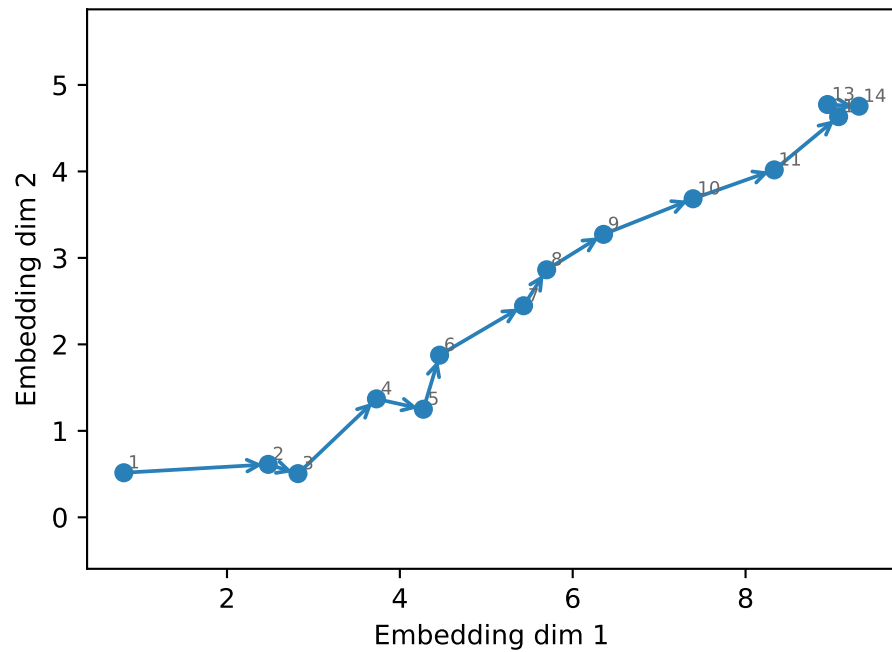
Pretrained LTC_step high, LTC_dir > 0
