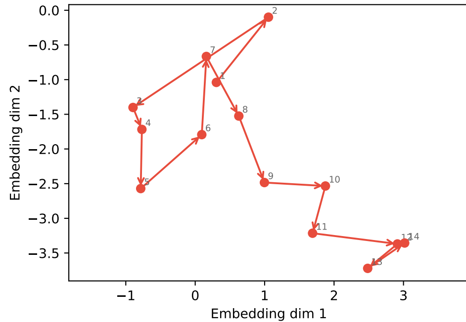
Random-weight LTC_step low, LTC_dir \sim 0
